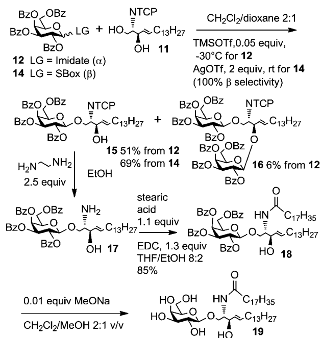
Scheme 5. Glycosylation of Acceptor 11 and Synthesis of Galactocerebroside
