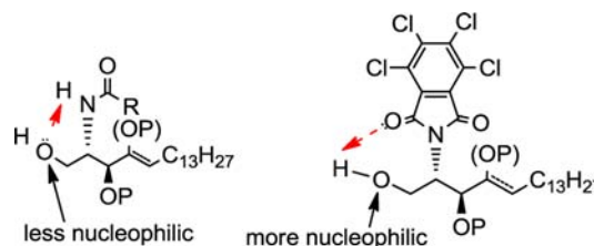
Figure 1. Hydrogen bonding in sphingosines.
