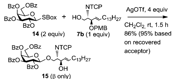
Scheme 4. Glycosylation of Acceptor 7b
