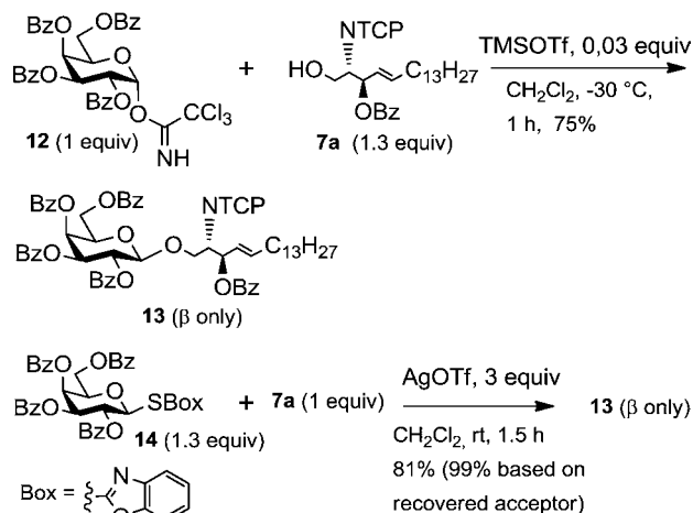
Scheme 3. Glycosylations of Acceptor 7a
