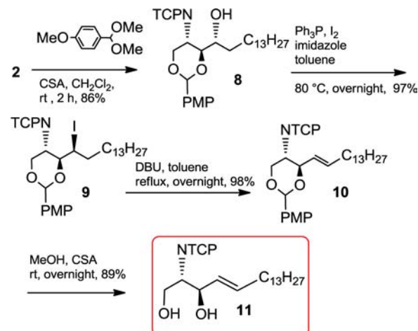
Scheme 2. Second Synthesis of a Sphingosine Acceptor
