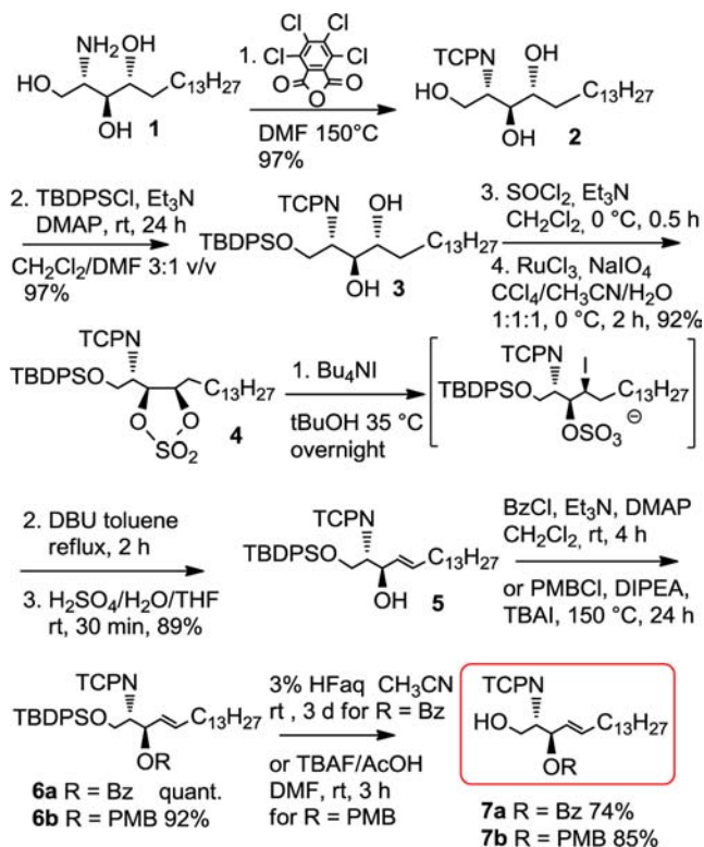
Scheme 1. First Synthesis of Sphingosine Acceptors
